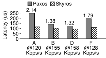
Figure 12. SKYROs Latency Benefits. The figure compares the average latency at maximum throughput for mixed YCSB workloads. The number below each bar shows the throughput for the workload.
